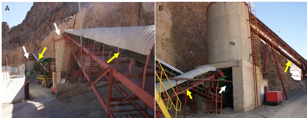
Figure 16: A) Conveyors (yellow arrows) and the coarse storage bins with a cone crusher crushers at the base (white arrows). B) A close-up view of the secondary crusher (white arrow).
