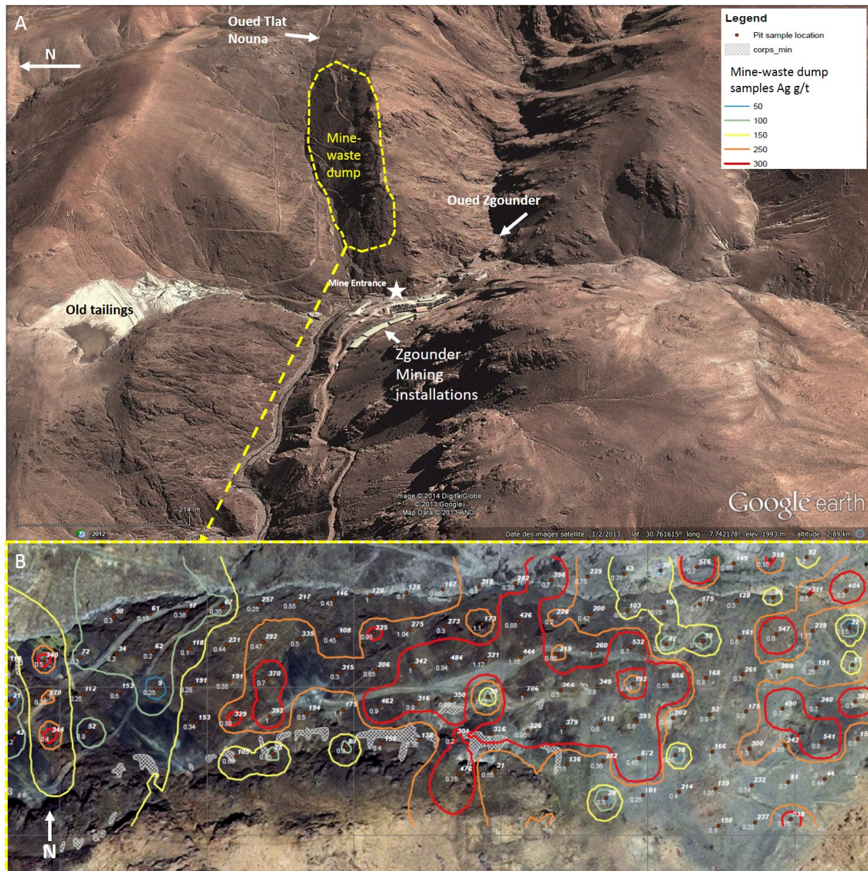
Figure 24: A) Location of the mine waste dump at the Zgounder silver mine (from Google Earth). B) Location of samples collected by BRPM from the mine waste dump.
