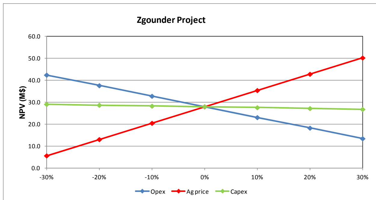
Figure 106: Graph of Sensitivity Analysis (NPV)
