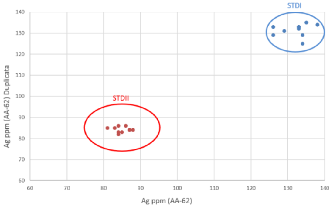
Figure 70: Custom standards STDI and STDII and their duplicate analyses
