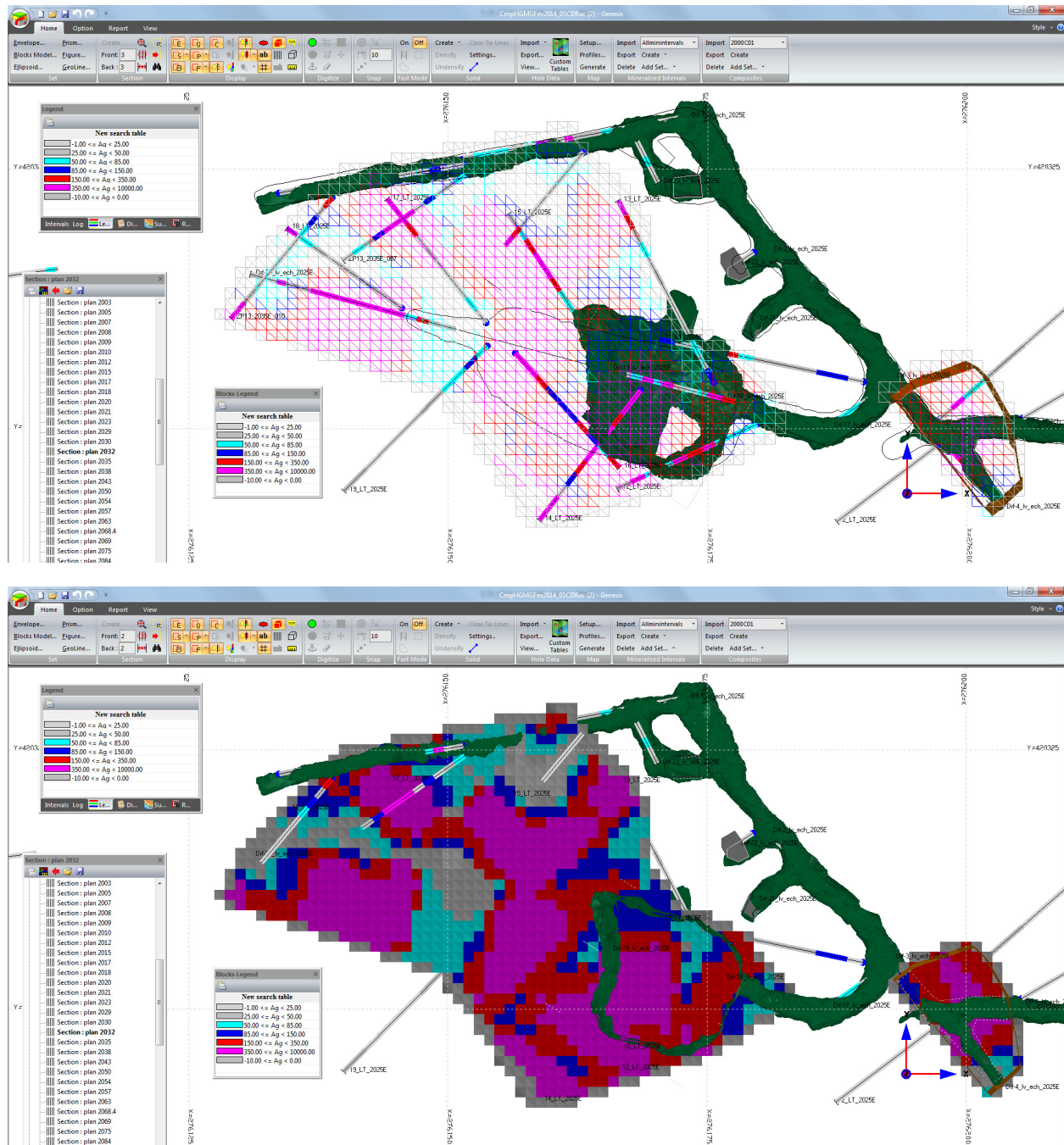
Figure 88: Example of block model Z2035A & Z2035C on level 2032 with openings
