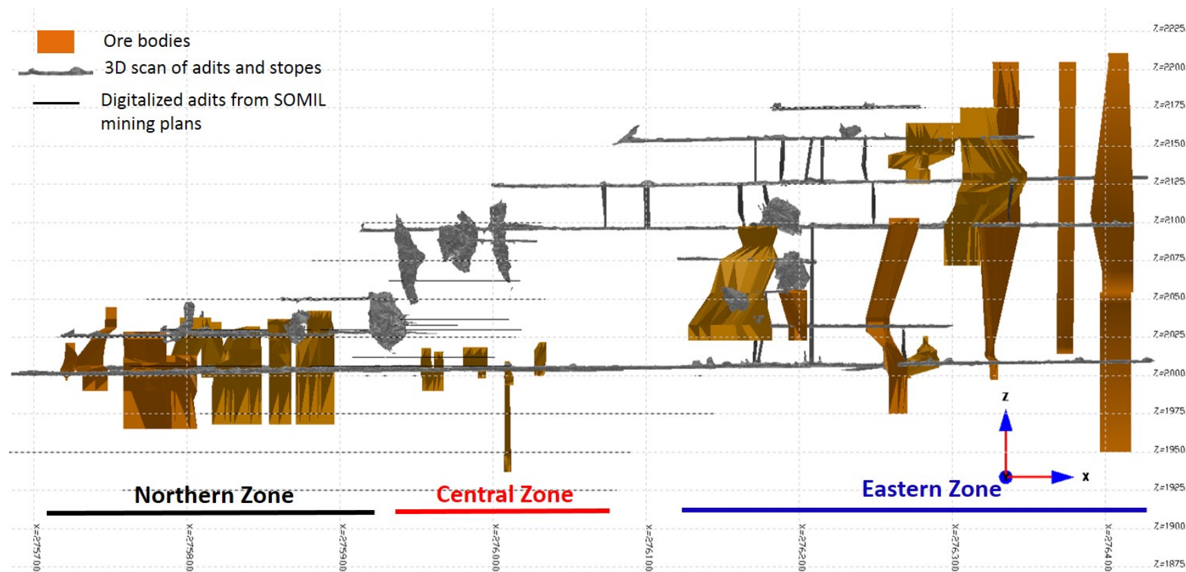
Figure 82: Long view looking North of the mineralized envelopes at Zgounder silver mine (northern, central and eastern zone)
