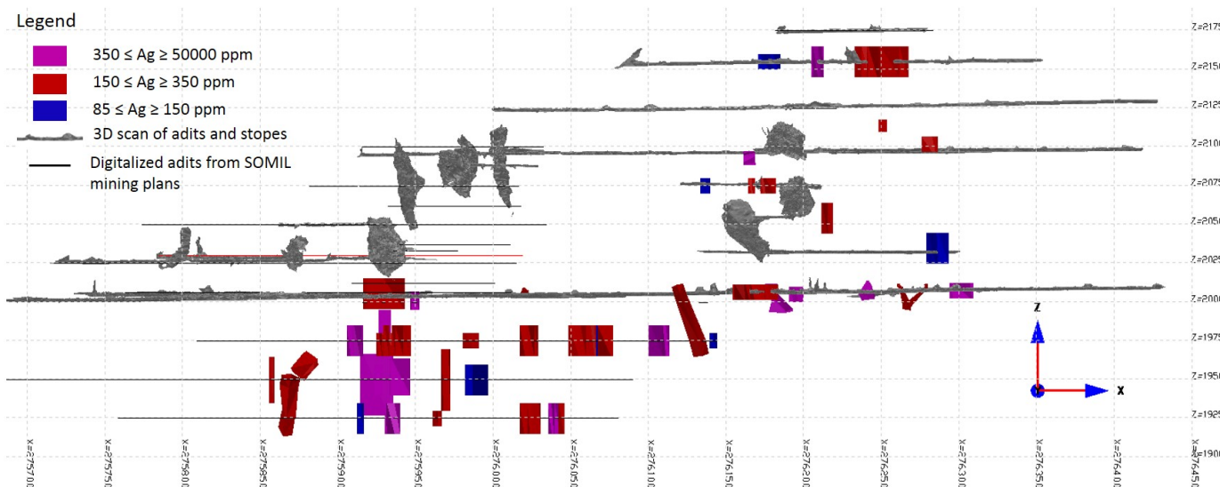
Figure 90: Localization of inferred panels between level 1925 and 2150m at the Zgounder silver mine
