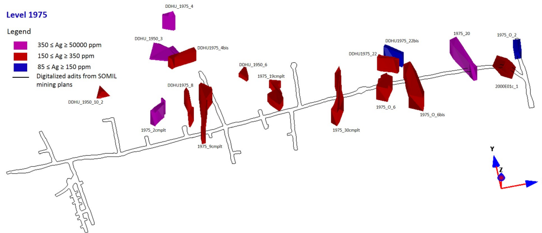
Figure 93: Localization of resources panels at level 1975, Zgounder silver mine
