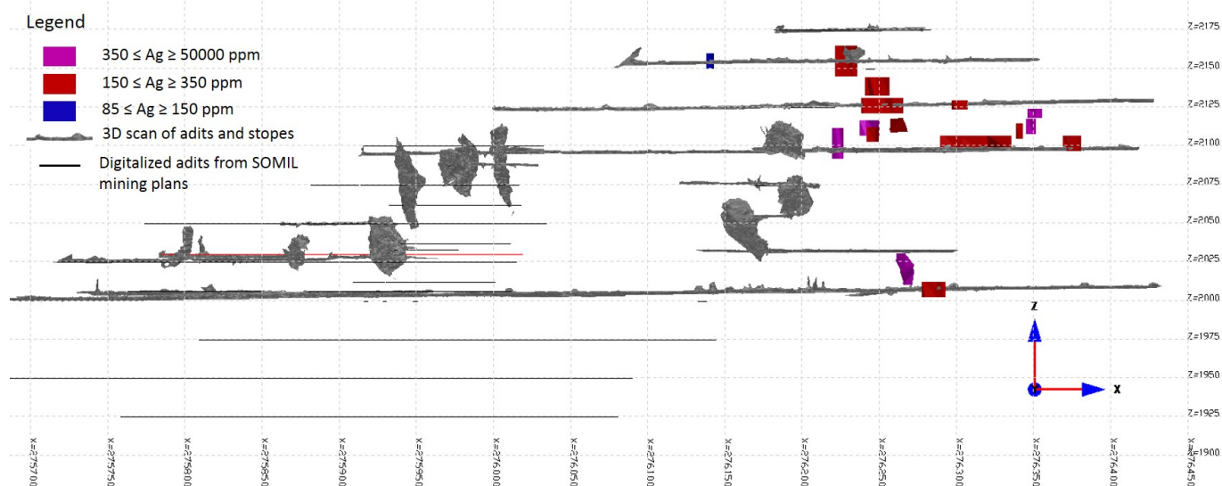
Figure 89: Localization of indicated panels between level 2000 and 2150m at the Zgounder silver mine
