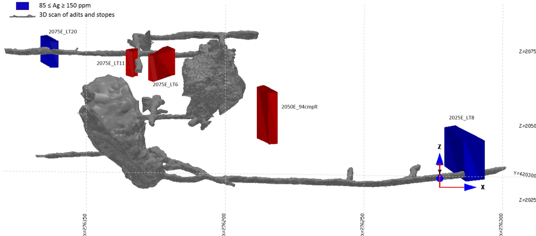
Figure 95: Localisation of resources panels at level 2035E, 2050E & 2075E, Zgounder mine
