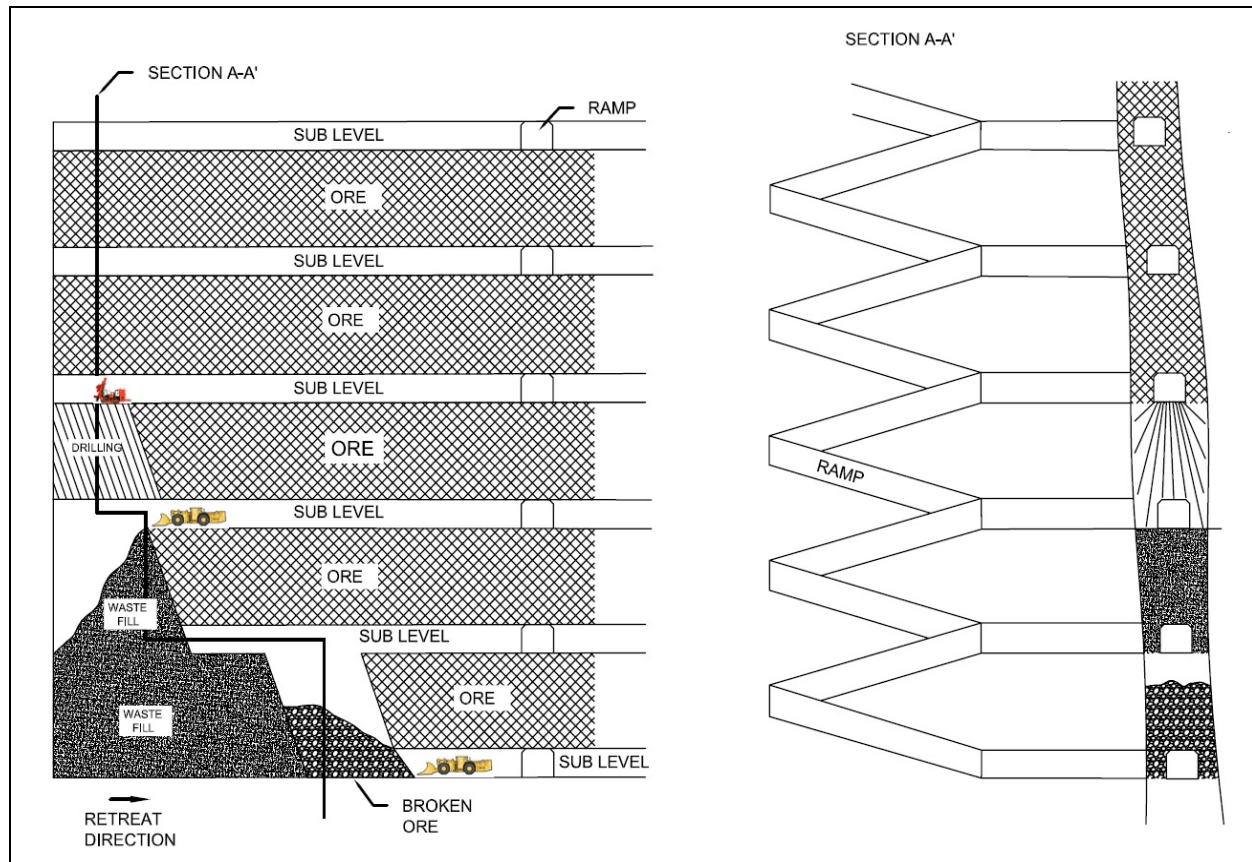
Figure 100: Avoca mining method - option 1
