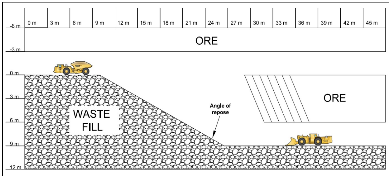
Figure 101: Avoca mining method - option 2
