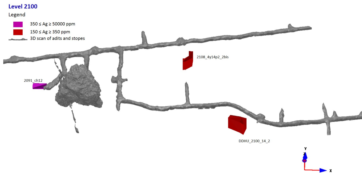
Figure 96: Localization of resources panels at level 2100, Zgounder silver mine
