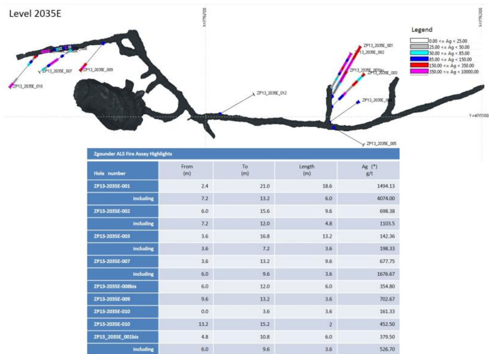
Figure 62: Twelve percussion holes drilled at the 2035E level with the highlights of the ALS fire assays.
