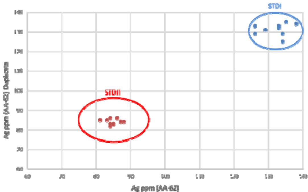
Figure 70: Custom standards STDI and STDII and their duplicate analyses.
