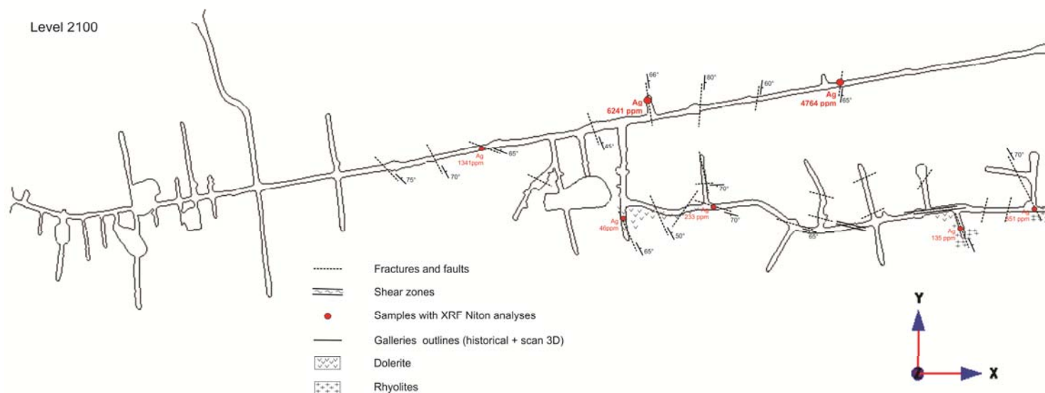
Figure 43: Distribution of fractures/faults and samples collected by GMG at the 2100 level, Zgounder silver mine.
