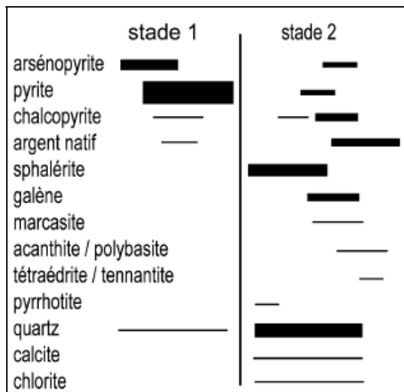
Figure 34: Paragenetic sequence of Zgounder deposit (From Marcoux & Wadjinny, 2005).
