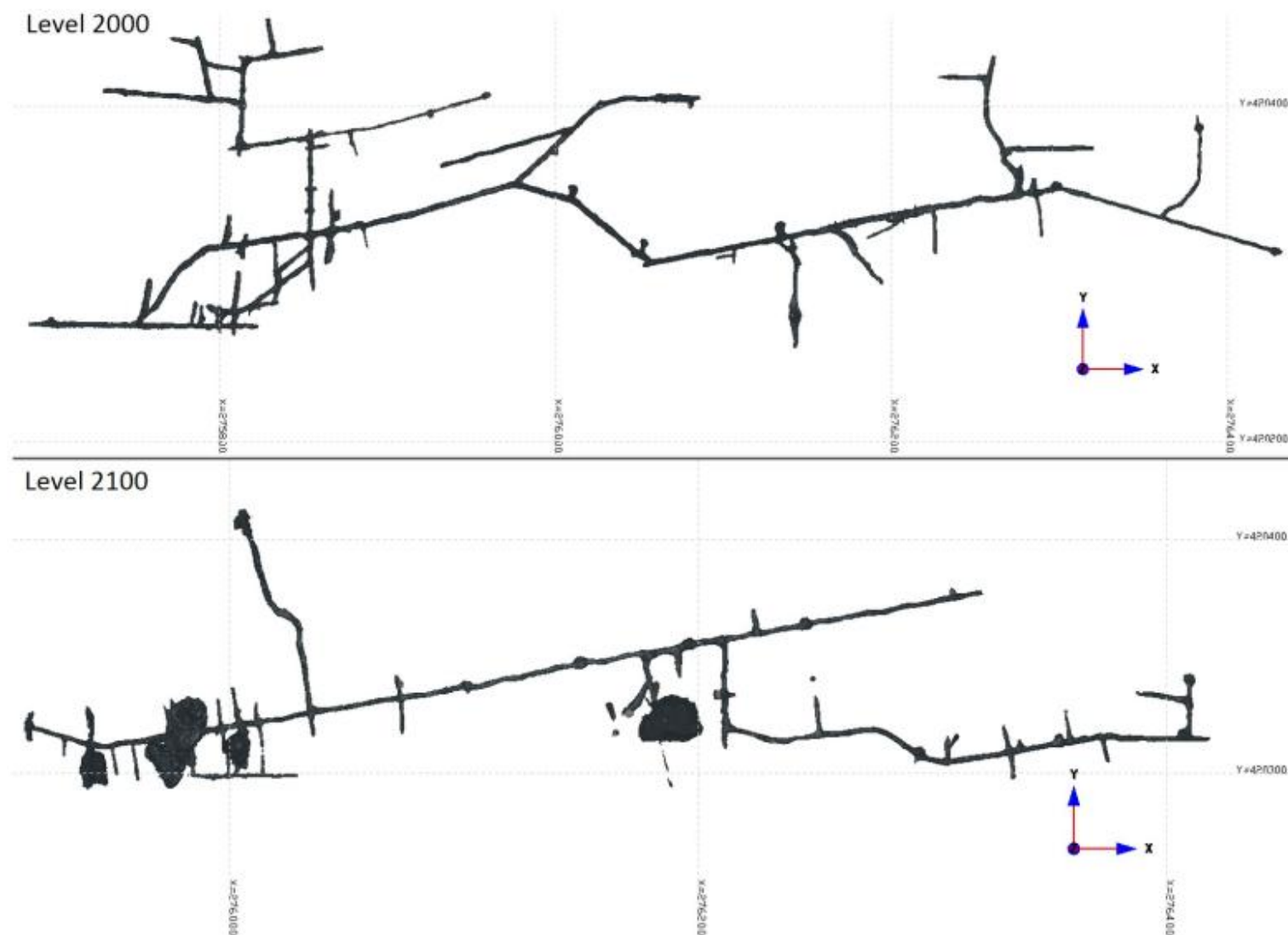
Figure 52: Plan views of the 3D scans for the 2000 and 2100 levels.
