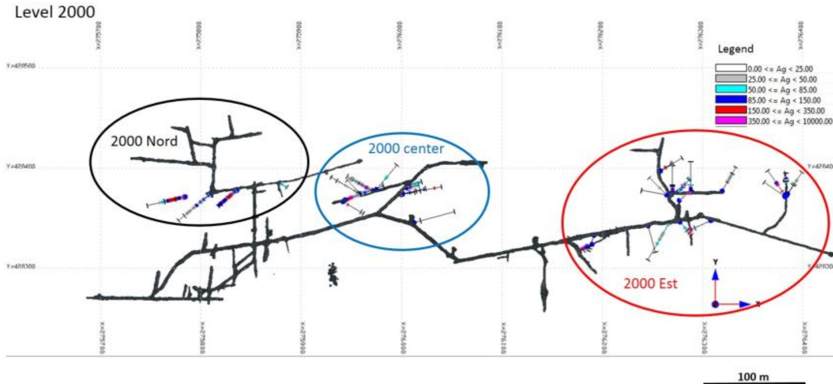
Figure 58: Plan view of the percussion drillholes at the 2000 level.
