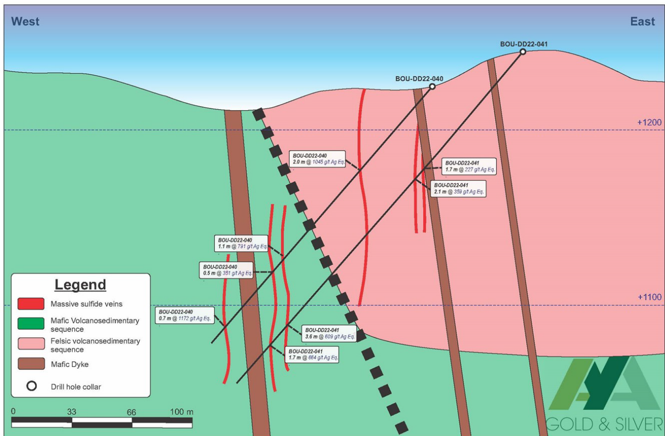
Figure 7-9 Cross-Sectional Projection 3,477,070 N of the Central Zone
