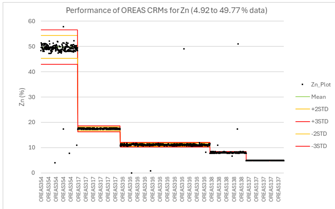
Figure 11-9 Performance of OREAS CRMs for Zn (4.92 to 49.77% data)
