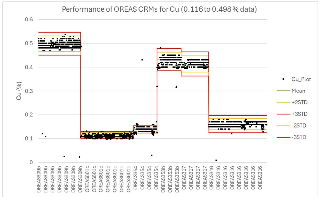
Figure 11-10 Performance of OREAS CRMs for Cu (0.116 to 0.498 % data)
