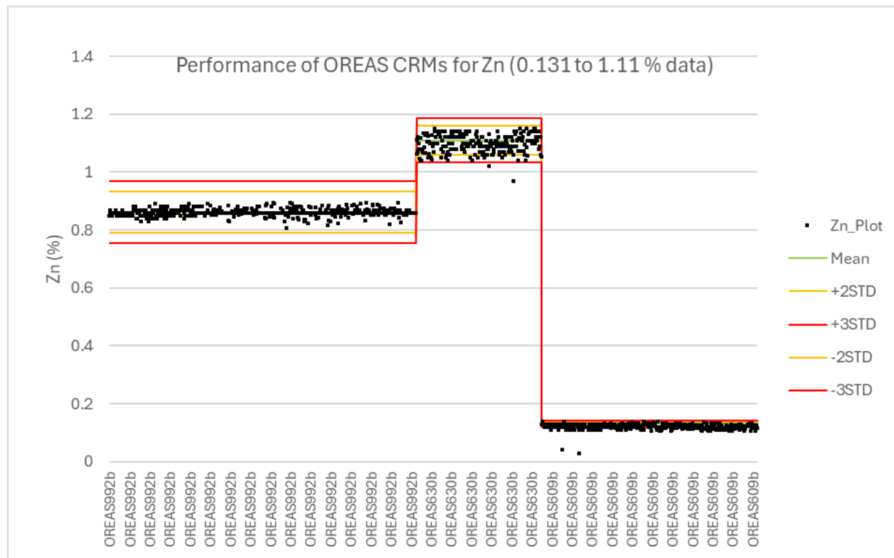
Figure 11-8 Performance of OREAS CRMs for Zn (0.131 to 1.11% data)
