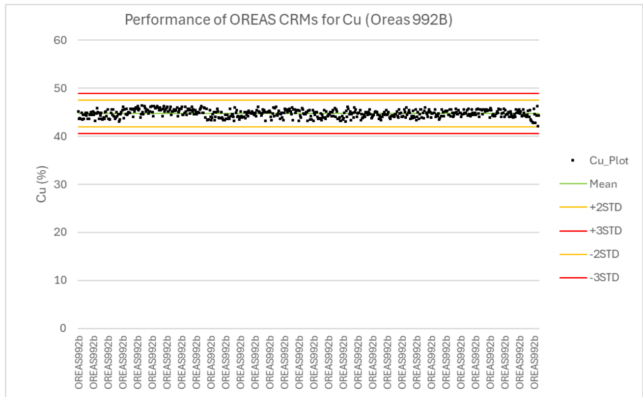
Figure 11-11 Performance of OREAS CRMs for Cu (oreas 992b)
