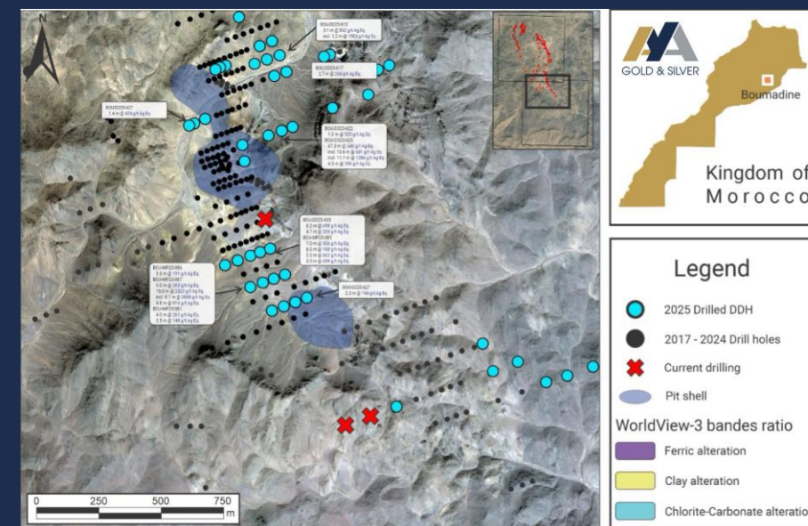
Figure (Right) : Surface Plan of Boumadine South Zone with New DDH Results
