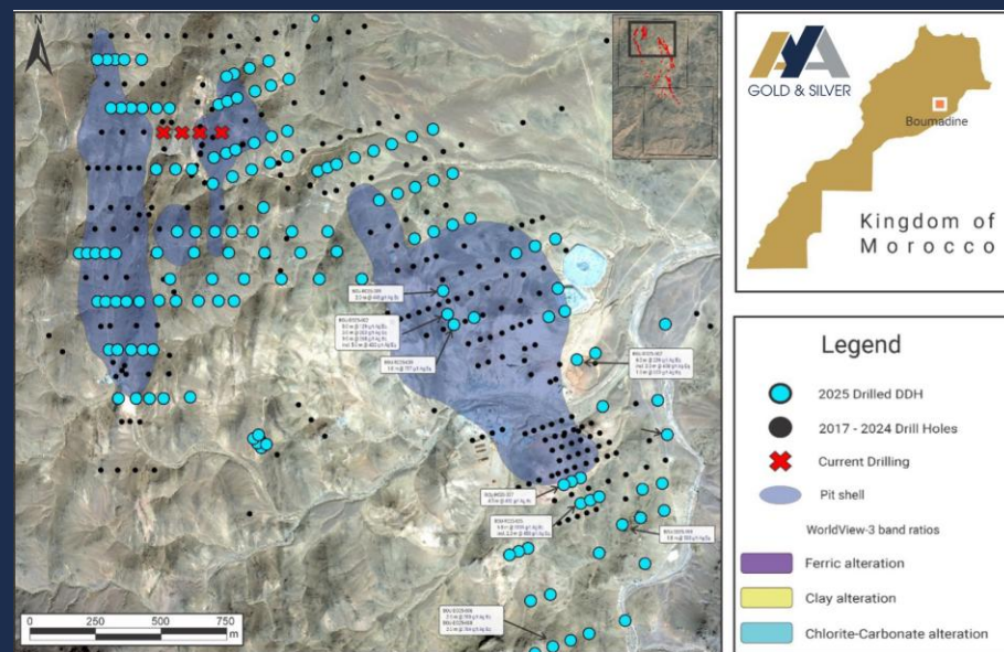
Figure (Left) : Surface Plan of Boumadine North, Imariren and Tizi Zones with New DDH Results
